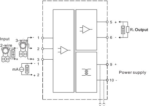
Single current input, single current/voltage output
