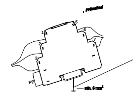
Connection diagram
